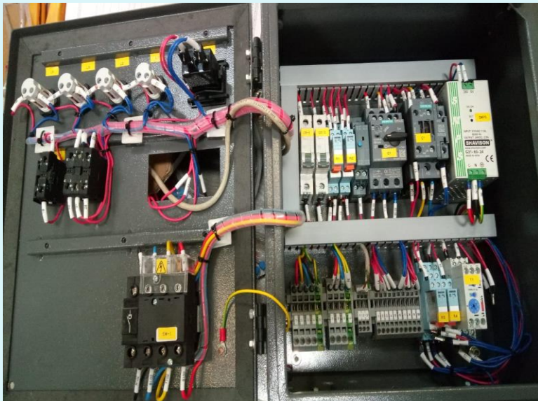
● LT PANEL
